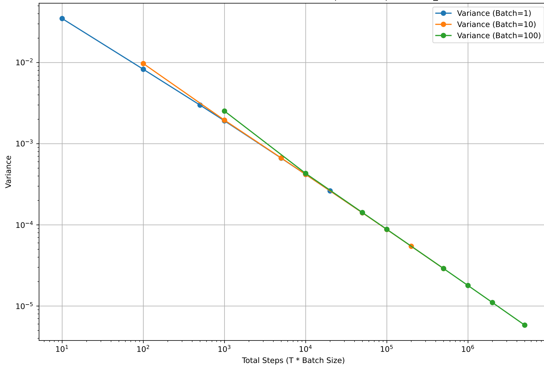
Slock Biases and Variances for Different Batch Sizes; \alpha=2.5 . optiized eta_star for each T
